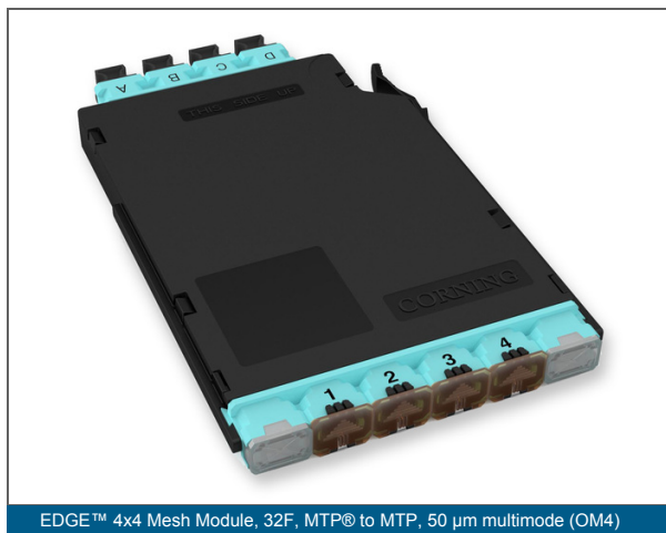
EDGE™ 4x4 Mesh Module, 32F, MTP® to MTP, 50 µm multimode (OM4)
